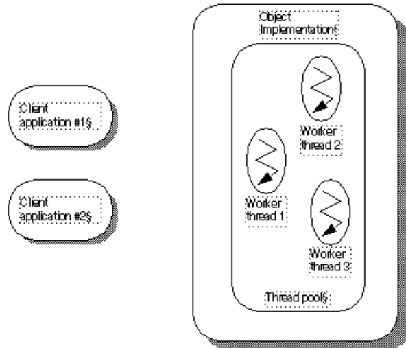
Figure 10.1 Pool of threads is available
