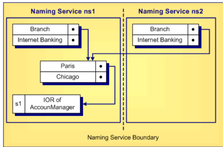
Figure 16.3 Naming contexts with multiple access hierarchies
