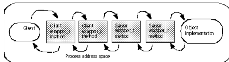
Figure 26.5 Typed object wrapper invocation order
