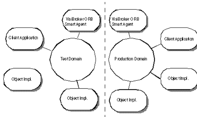
Figure 14.1 Running separate VisiBroker ORB domains simultaneously
