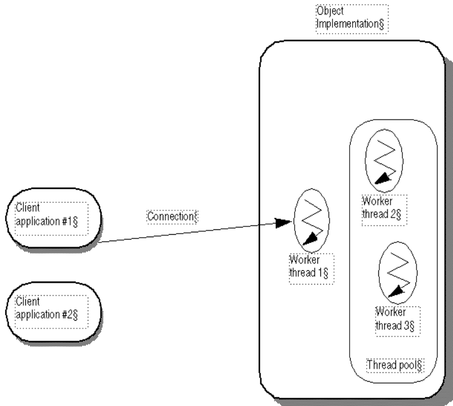
Figure 10.2 Client application #1 sends a request
