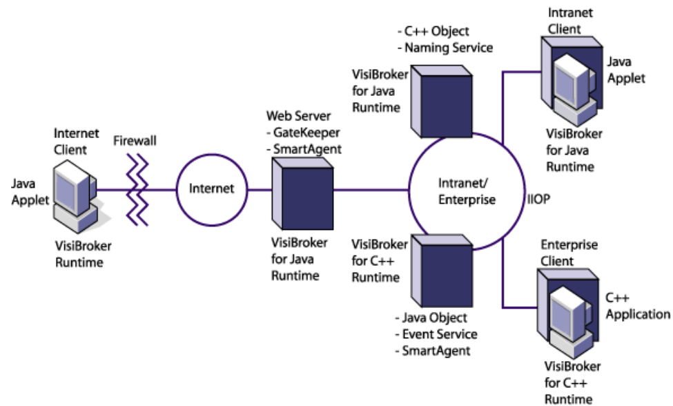
Figure 2.2 VisiBroker Architecture
