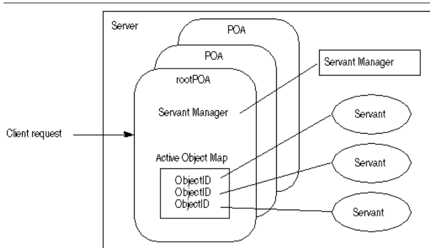
Figure 9.1 Overview of the POA
