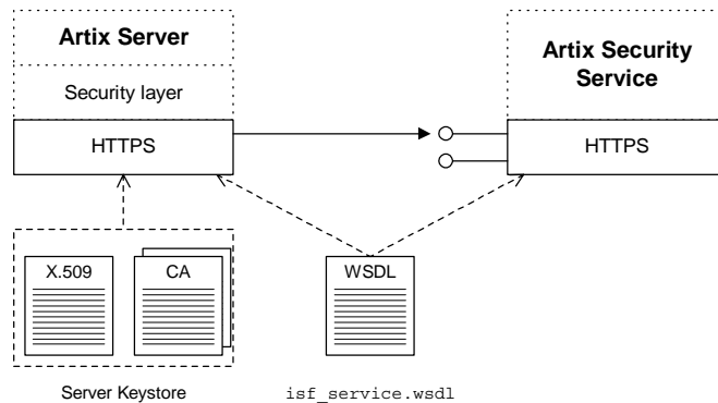
Figure 37: Overview of Connecting to the Security Service
