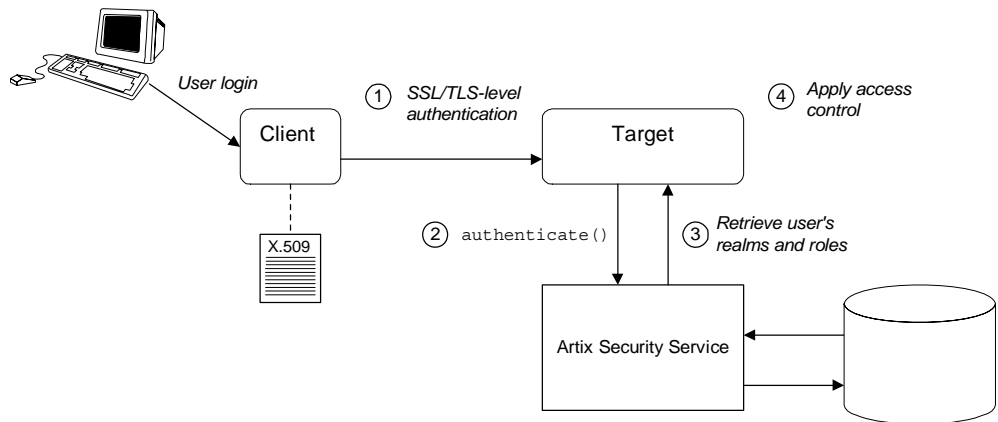
Figure 15: Overview of Certificate-Based Authentication with HTTPS—Java Runtime
