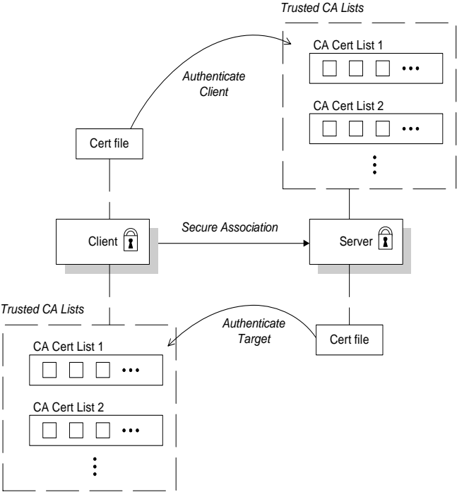
Figure 27: Mutual Authentication
