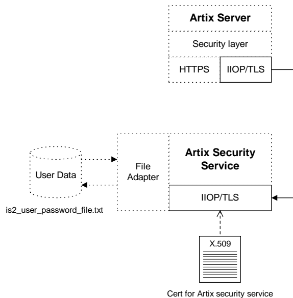
Figure 7: An IIOPTLS Connection in the HelloWorld Example
