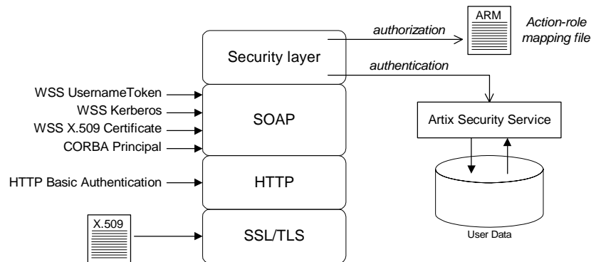
Figure 17: Overview of Security for SOAP Bindings
