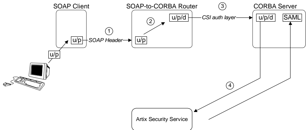
Figure 50: Propagating Credentials Across a SOAP-to-CORBA Router
