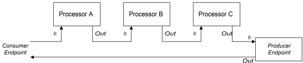
Figure 5. Sample Pipeline for InOut Exchanges
