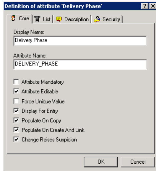
Figure 3-12. Attribute Definition
