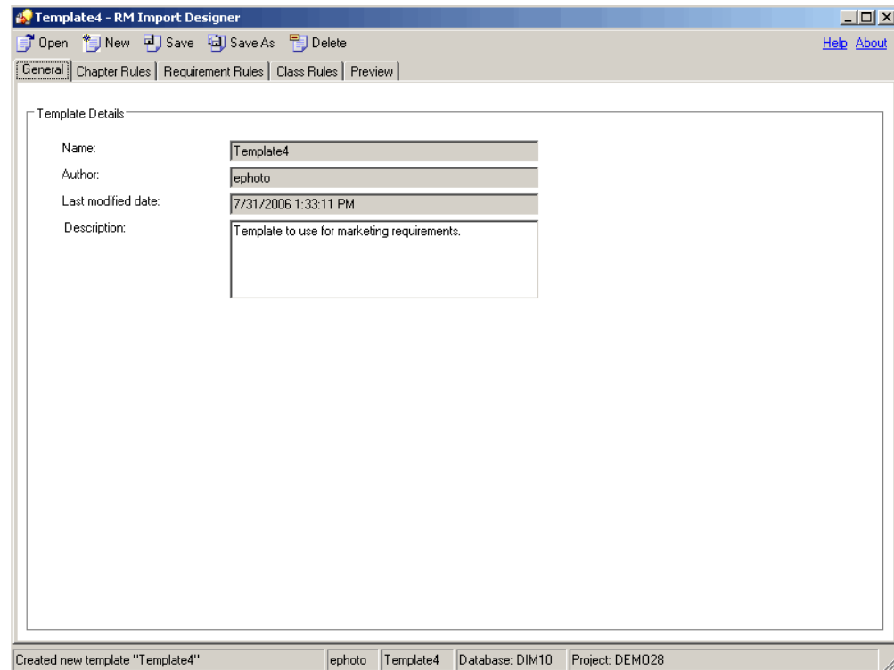
Figure 6-4. General Tab
