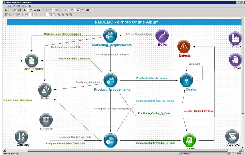
Figure 1-4. Class Definition
