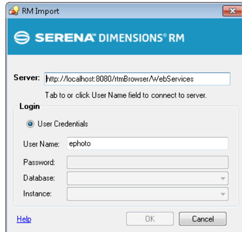
Figure 10-1. Login Dialog
