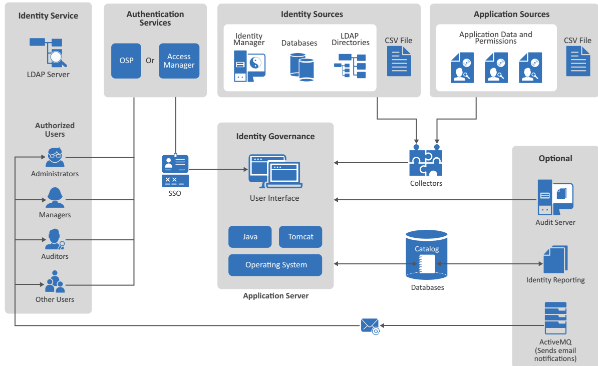
Figure 1-1 Overview of the OpenText Identity Governance Components
