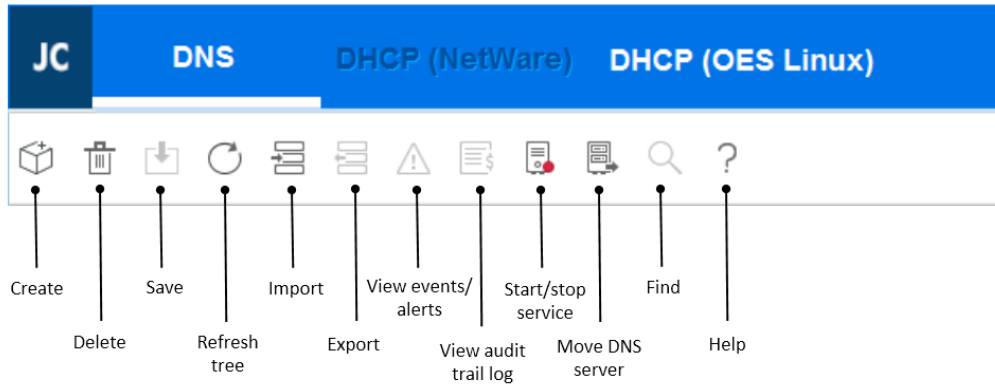
Figure 1-13 Toolbar
