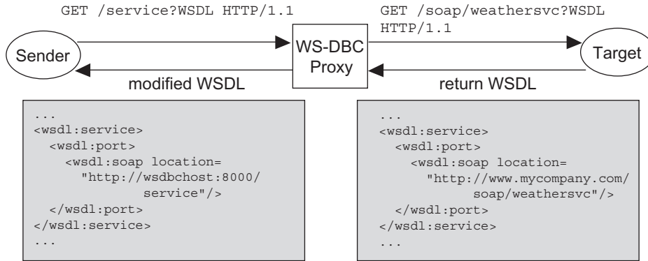
Fig. 13. WSDL modified by the WS-DBC Proxy
