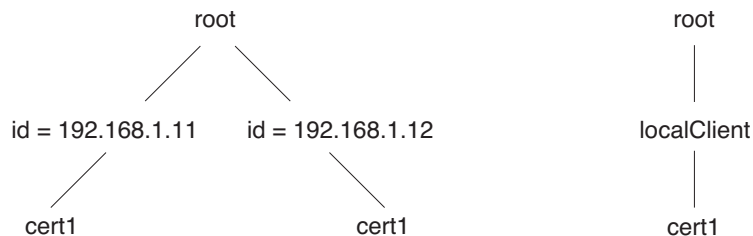
Fig. 8. Access Session Hierarchy
