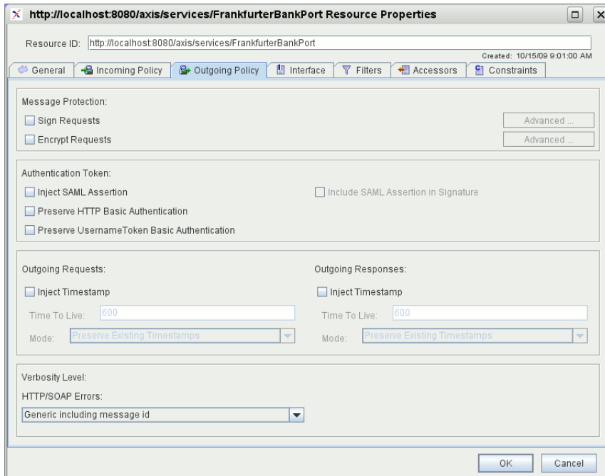
Fig. 31. Web Service Resource Properties: Outgoing Policy
