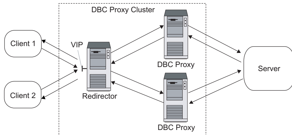
Fig. 10. Multiple WS-DBC Proxies, balanced load
