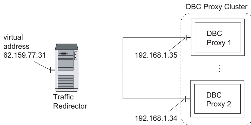
Fig. 30. External Interfaces and Virtual Address of DBC Proxies in a cluster
