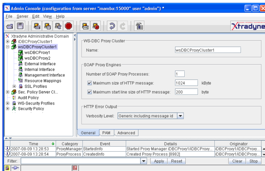
Fig. 23. WS-DBC Proxy Cluster Properties
