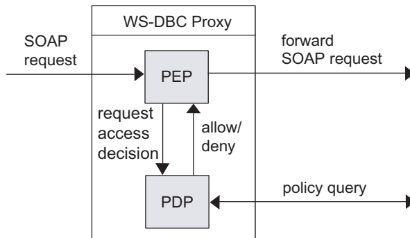
Fig. 7. WS-DBC Proxy functionality
