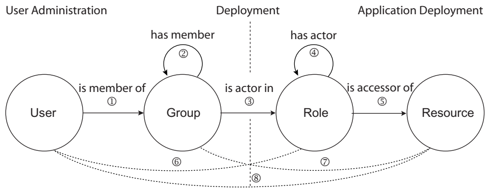
Fig. 1. Components of the access control policy
