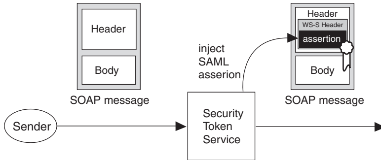
Fig. 5. Security Token Service adds a SAML assertion to a SOAP message
