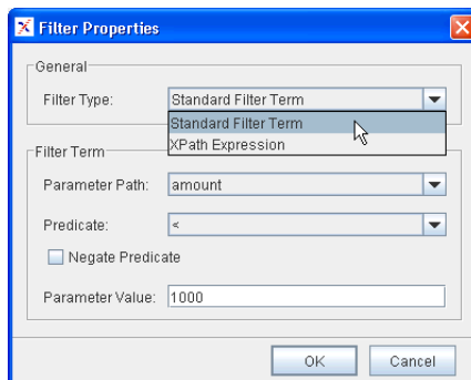
Fig. 38. Resource Properties: Defining Filter Properties
