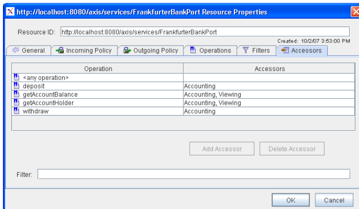
Fig. 49. FrankfurterBank Resource Accessor list
