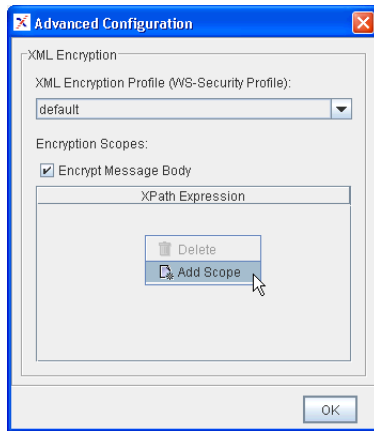
Fig. 33. Outgoing Policy: Encrypt Message – Advanced Configuration Properties
