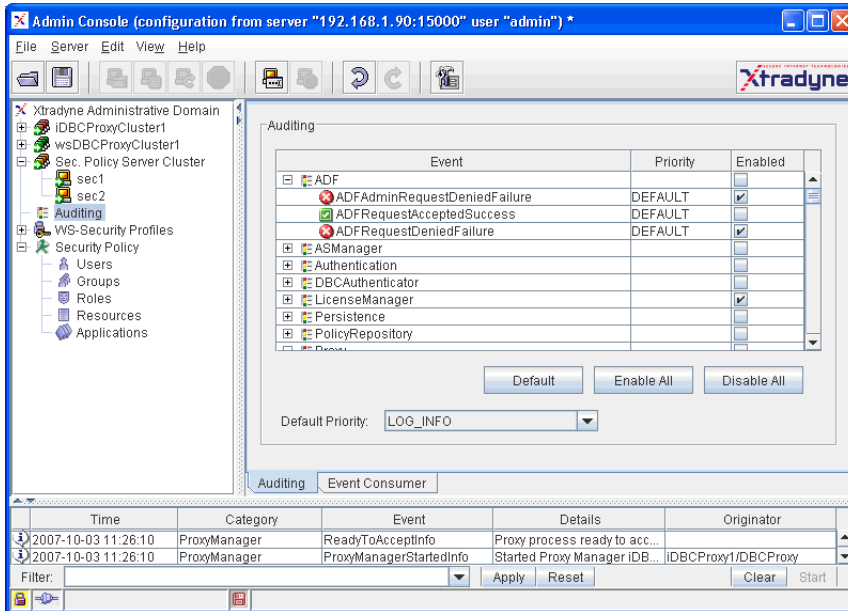
Fig. 57. Auditing – Configuring Audit Events
