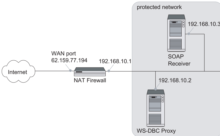
Fig. 2. The screened host firewall with WS-DBC Proxy
