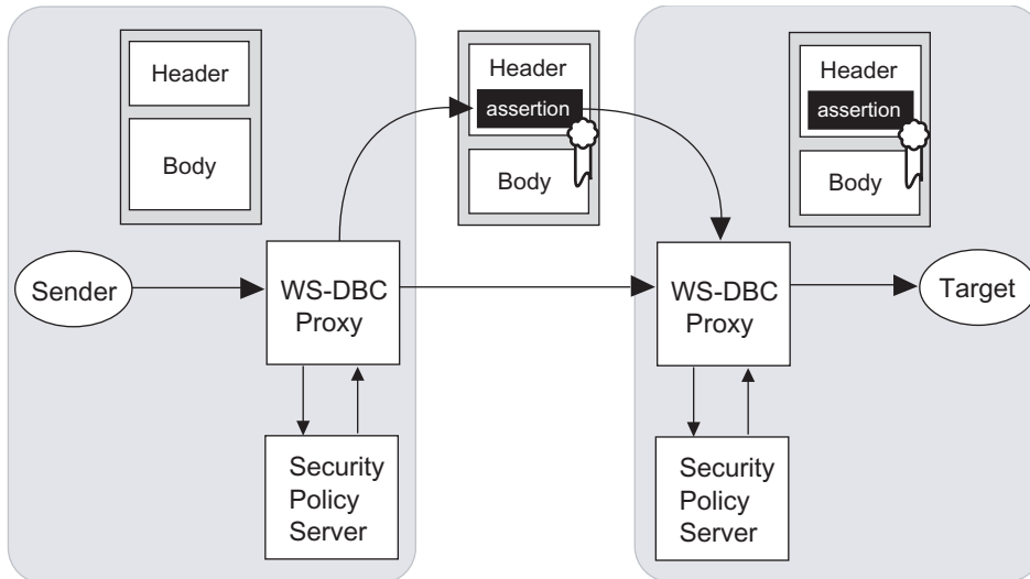
Fig. 12. A sender WS-DBC as an attribute authority.
