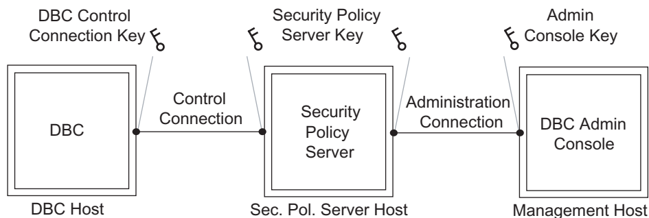
Fig. 63. Keys used on the Control and Administration Connection
