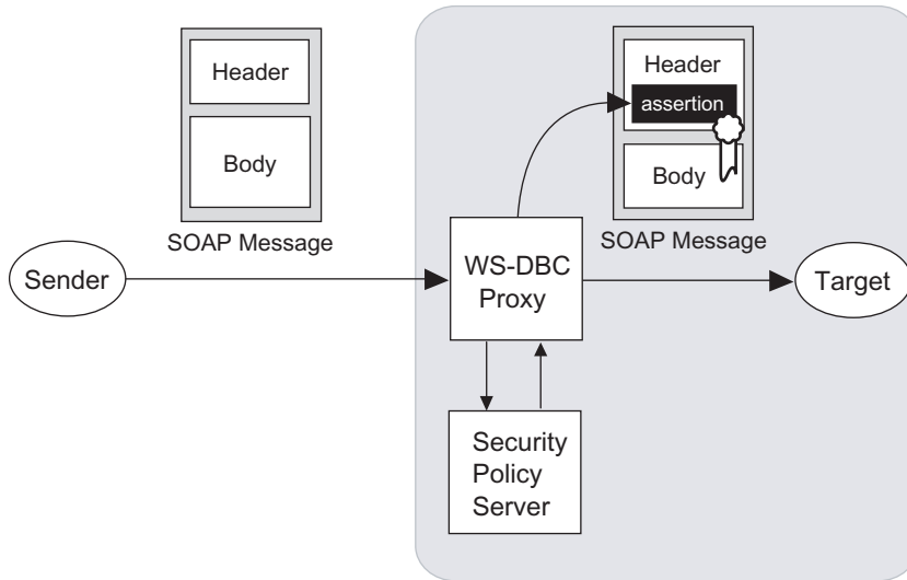
Fig. 11. A single, target-side WS-DBC
