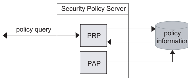
Fig. 8. Security Policy Server functionality
