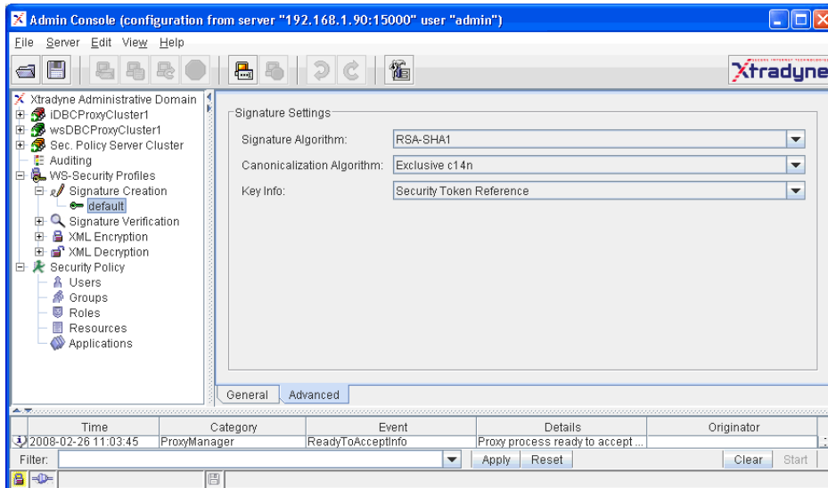
Fig. 49. Signature Creation Profile - Advanced Tab
