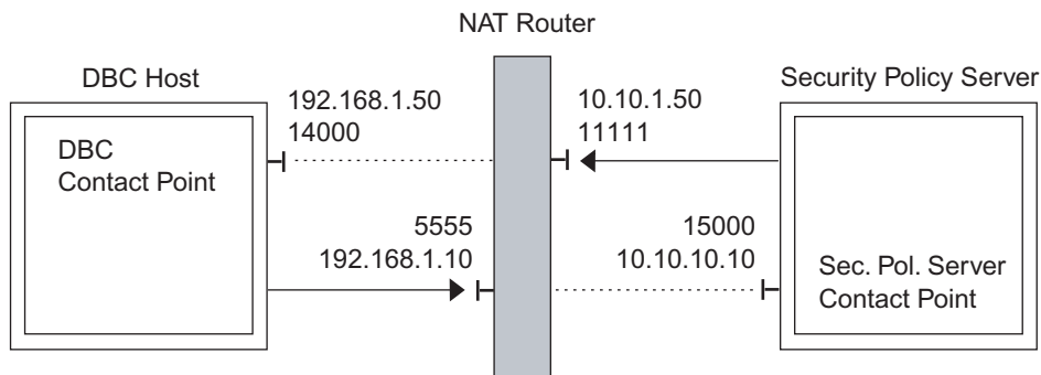
Fig. 56. NAT Router between the DBC Proxy host and the SPS host
