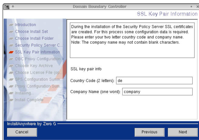
Fig. 7. SSL Key Pair information
