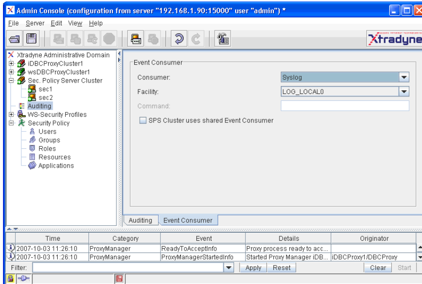
Fig. 58. Auditing – Configuring the Event Consumer
