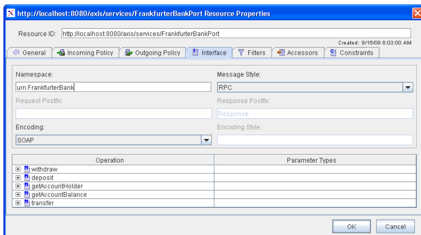
Fig. 34. Web Service Resource Properties: Interface
