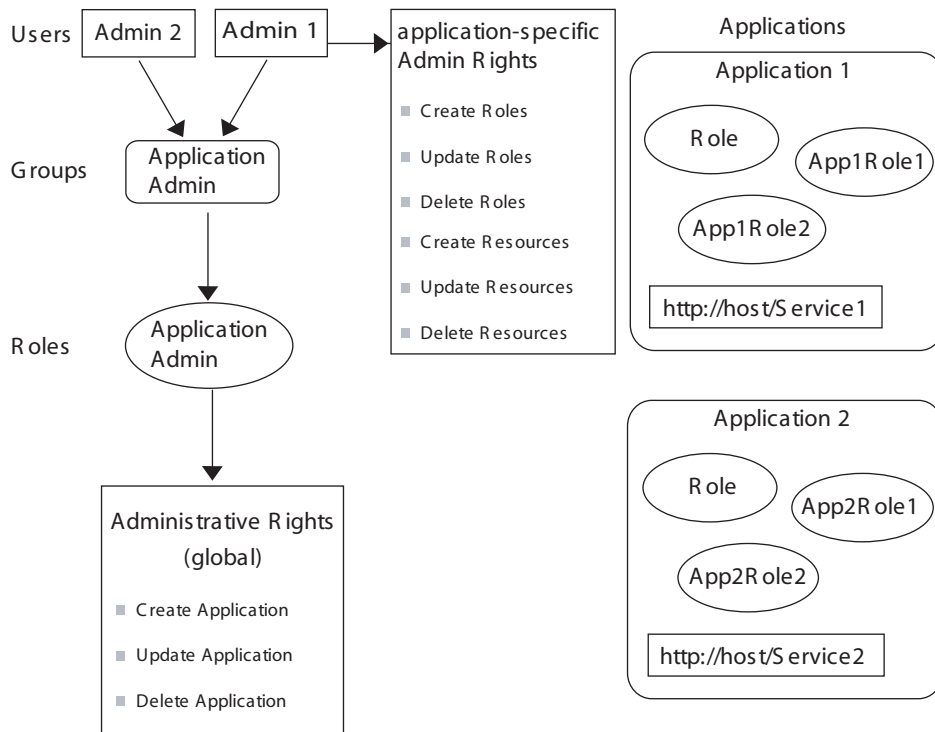
Fig. 43. Example Application Domains and administrative rights
