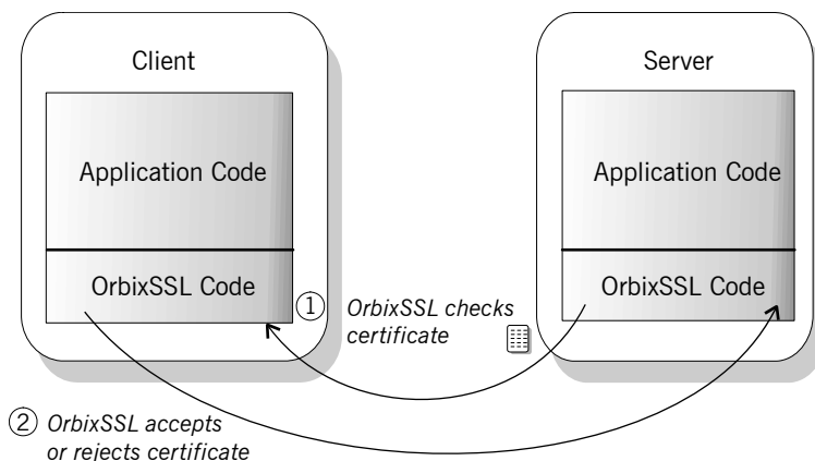
Figure 4 OrbixSSL Validating a Certificate
