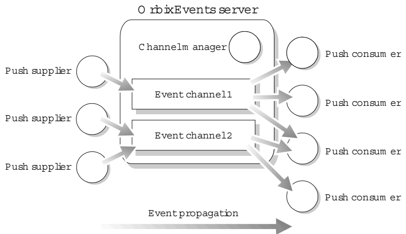
Figure 13 Example OrbixEvents Architecture with Two Event Channels
