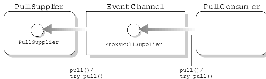
Figure 10 Transfer of an Event Through an Event Channel to a Consumer using the Untyped Pull Model
