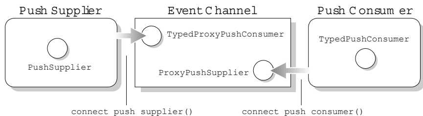
Figure 11 Push Supplier and Push Consumer Connecting to an Event Channel using the Typed Model
