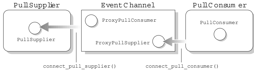
Figure 8 Pull Supplier and Pull Consumer Connecting to an Event Channel in the Untyped Model
