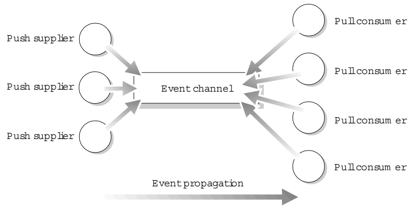
Figure 6 Push Model Suppliers and Pull Model Consumers in a Single System
