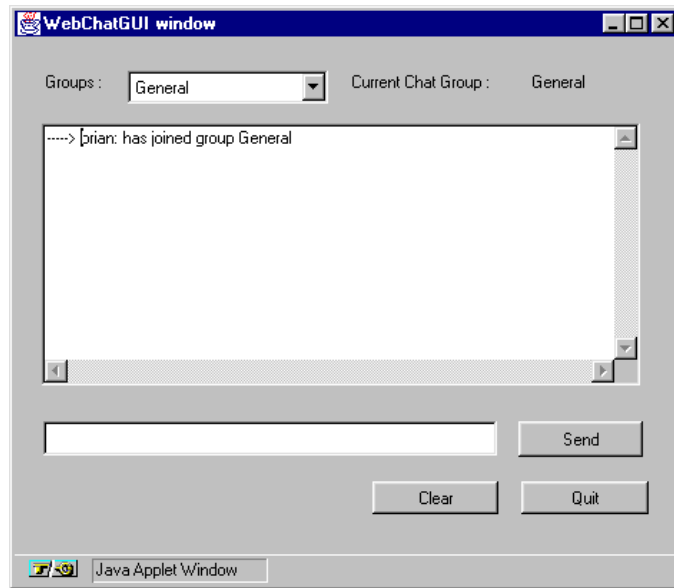
Figure 23 WebChat Client Interface
