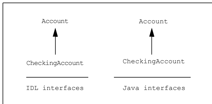
Figure 17 IDL and Java Inheritance Hierarchies
