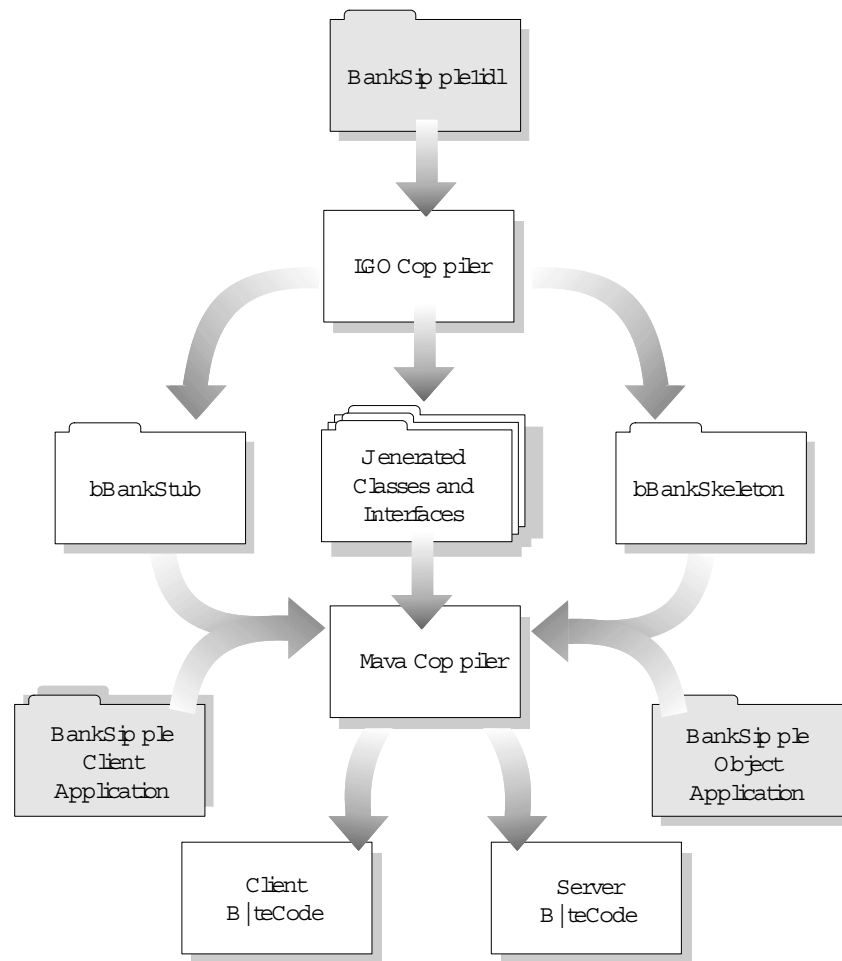
Figure 8 Overview of the Compiling the Bank IDL Interface
