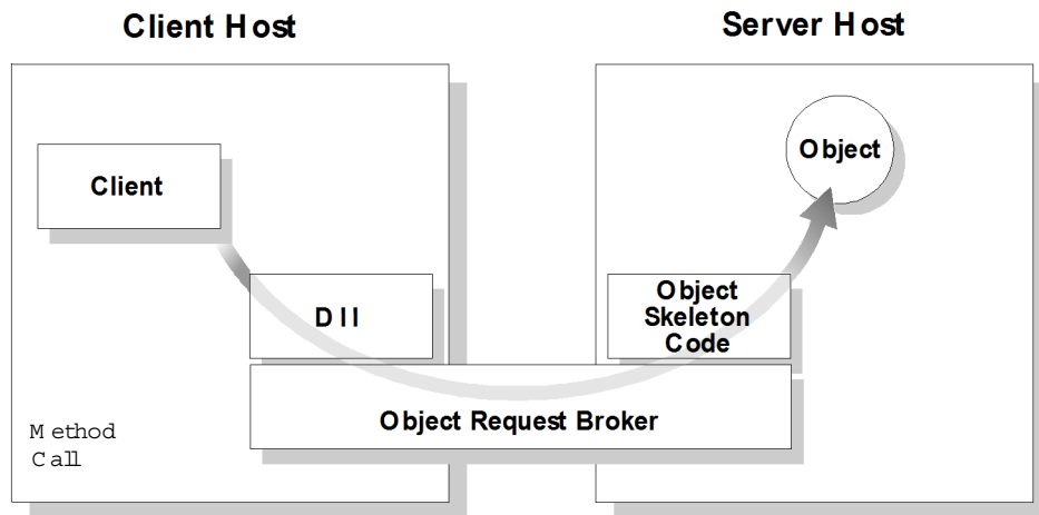
Figure 3 Client Invoking a Method Using the DII
