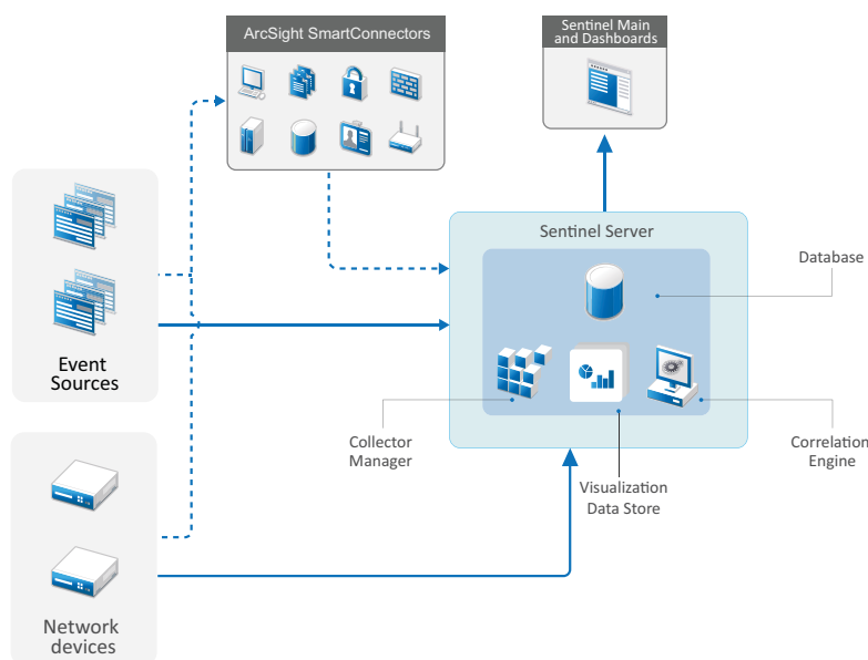
Figure 6-1 All-In-One Deployment
