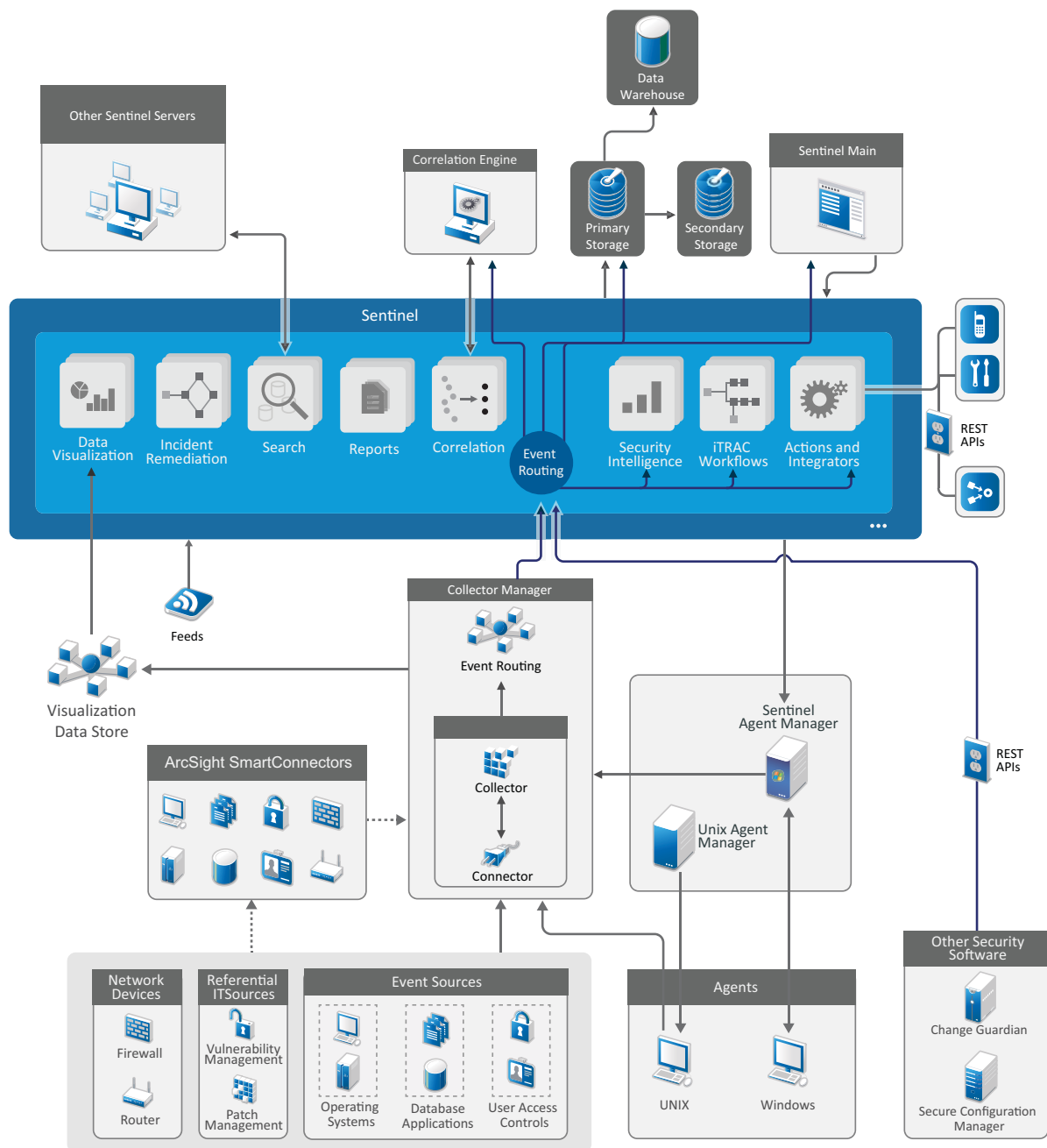
Figure 2-1 Sentinel Architecture
