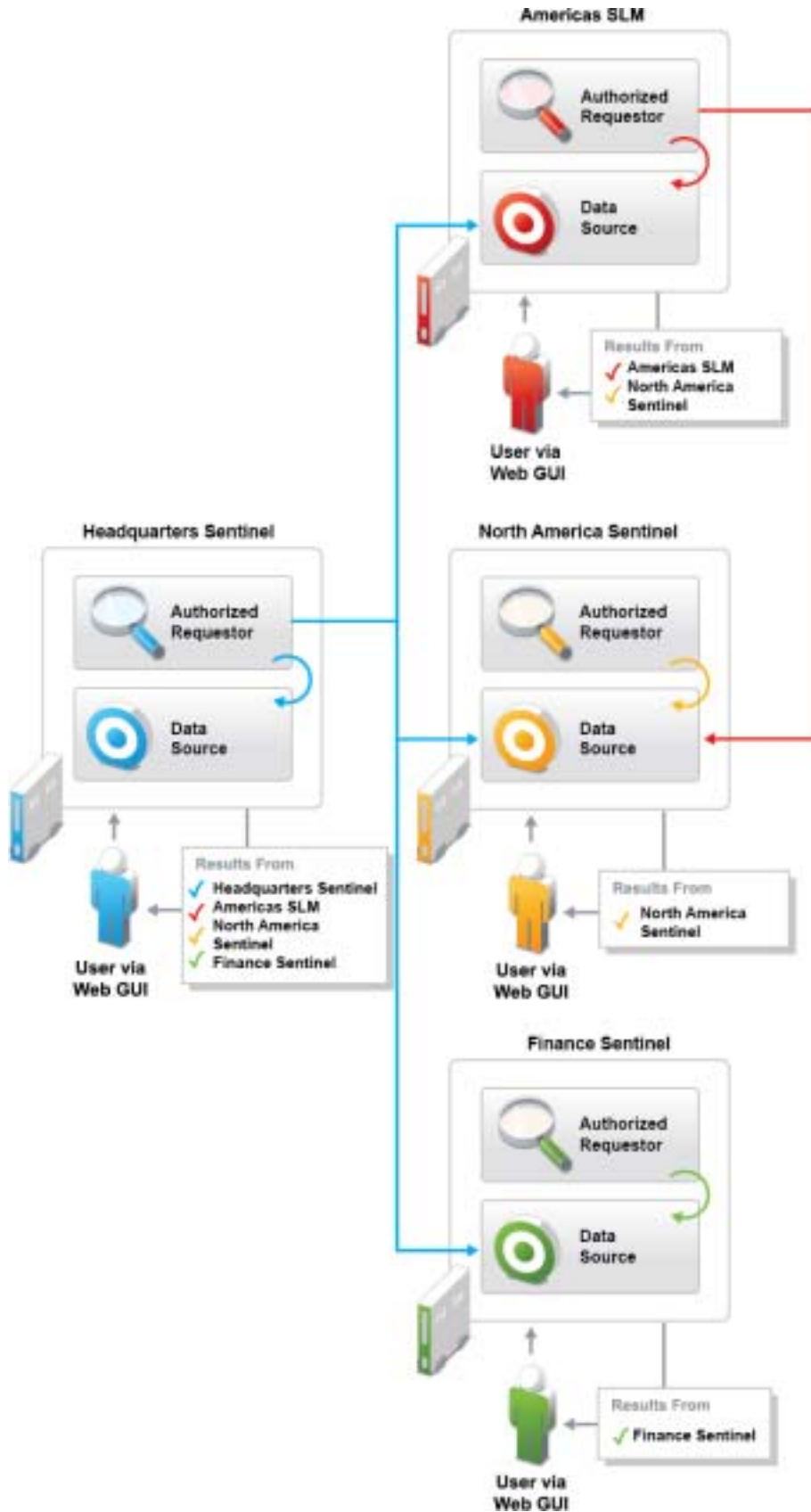
Figure 22-1 Data Federation
