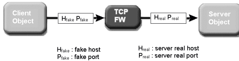
Figure 10 TCP firewall with NAT
