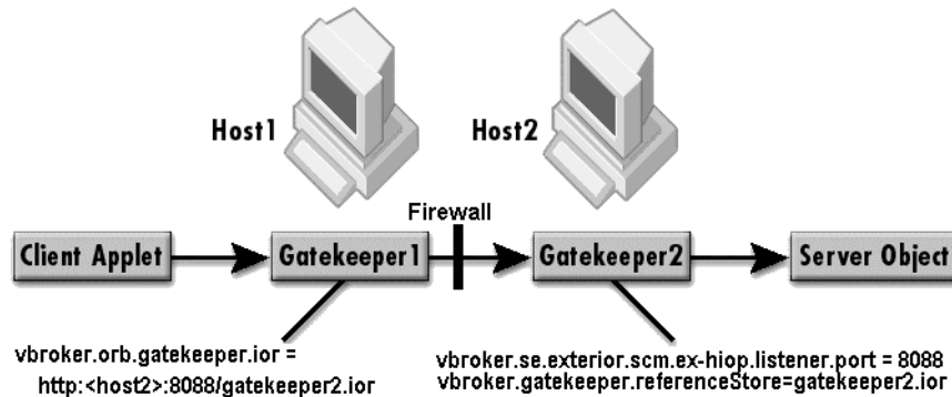
Figure 11 Static chaining of GateKeepers
