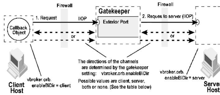
Figure 15 Callback with GateKeeper's bidirectional support
