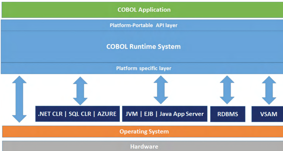
Figure 2. High performance, portable runtime execution environment for COBOL applications
