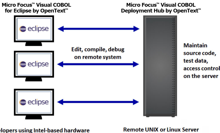
Figure 4. Micro Focus Visual COBOL for Eclipse remote development option
