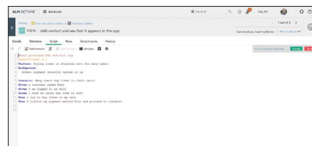
Figure 4. Gherkin test view within ALM Octane
