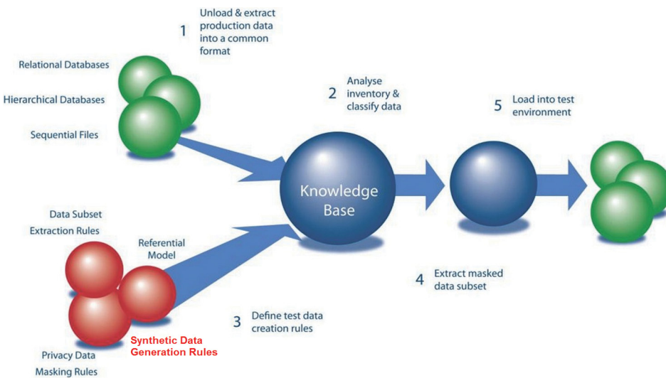
Figure 1. Strategic architecture for subsetting and masking with Data Express
