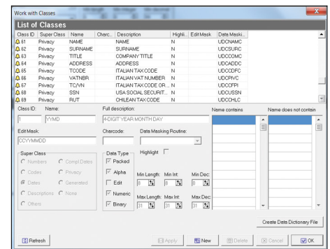
Figure 3. Class Definition with Data Express
