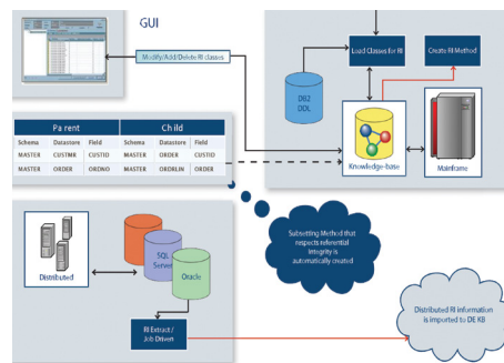
Figure 5. Cross-platform Complex Subsetting
