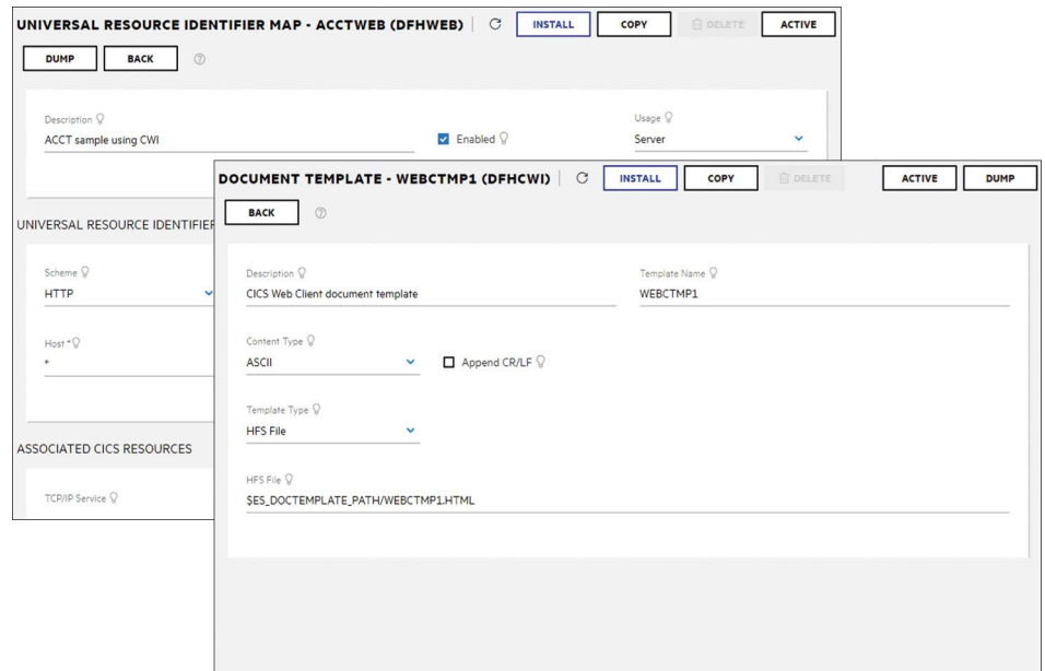
Figure 1. ESCWA UI simplifies configuration tasks
