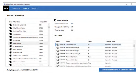
Figure 2. Cloud-readiness Assessment
