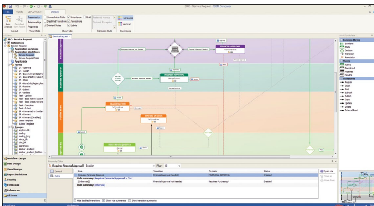
Figure 2. Graphically model and create process apps in SBM Composer.
