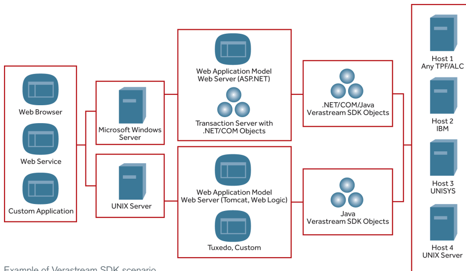
Example of Verastream SDK scenario.
